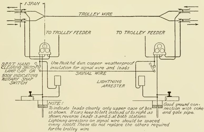
Fig. 214. Diagram of Automatic Block Signal System
